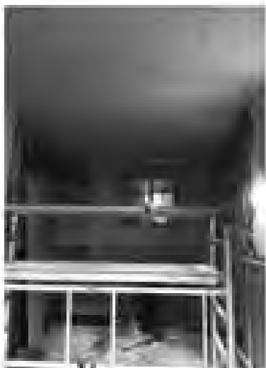
Ceiling Details: installation of new 1/2-inch fire-rated ceiling to underside of original ceiling structure and insulation (left), and finishes plasterboard (right)
